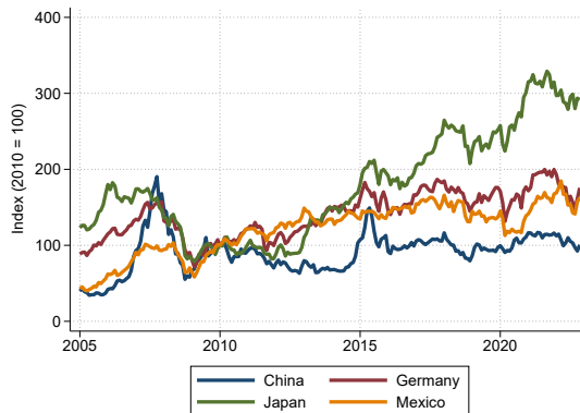
(e) CAPE for various countries
